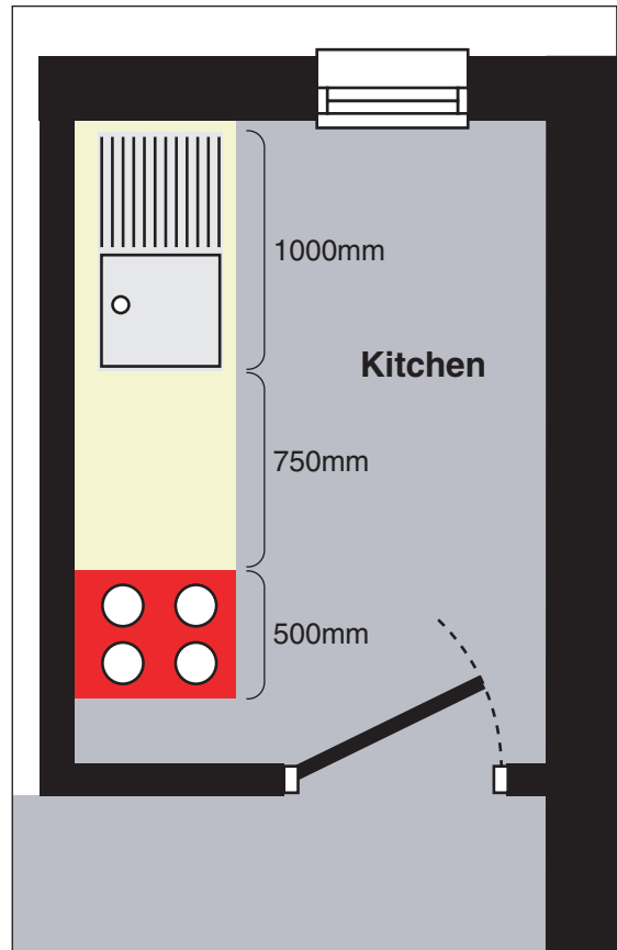
Floor layout
