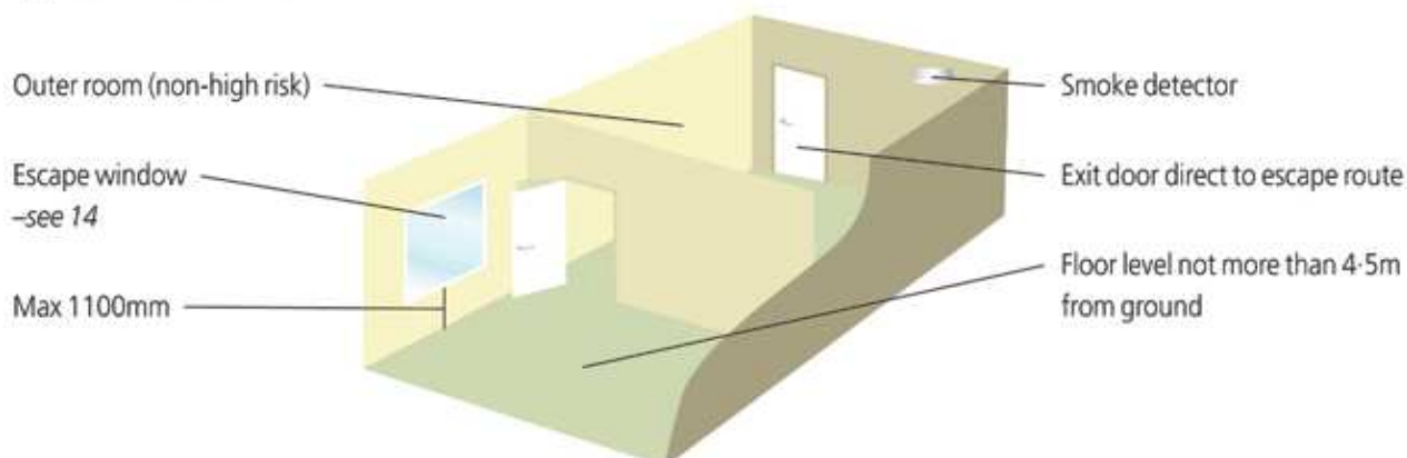
figure C3: inner rooms
